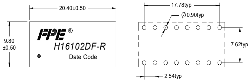
SUGGESTED PCB LAYOUT
